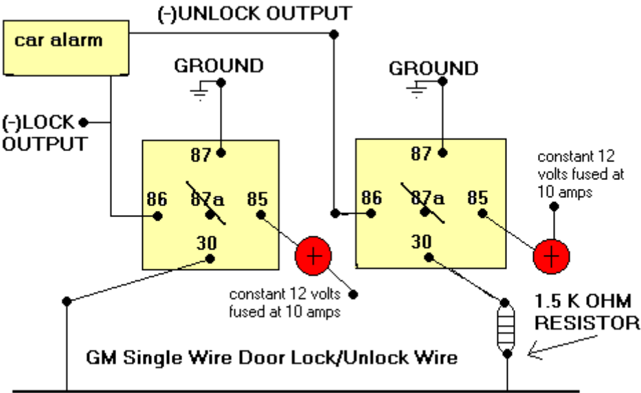
This diagram Shows The New 1999 Grand Am Single Wire Door lock/Unlock Solution
